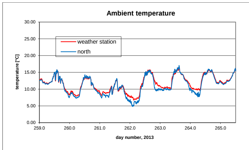
B11.16. Ambient temperature.
