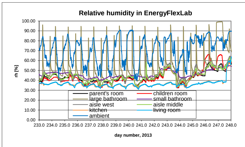
B9.2. Relative humidity in the house and ambient.
