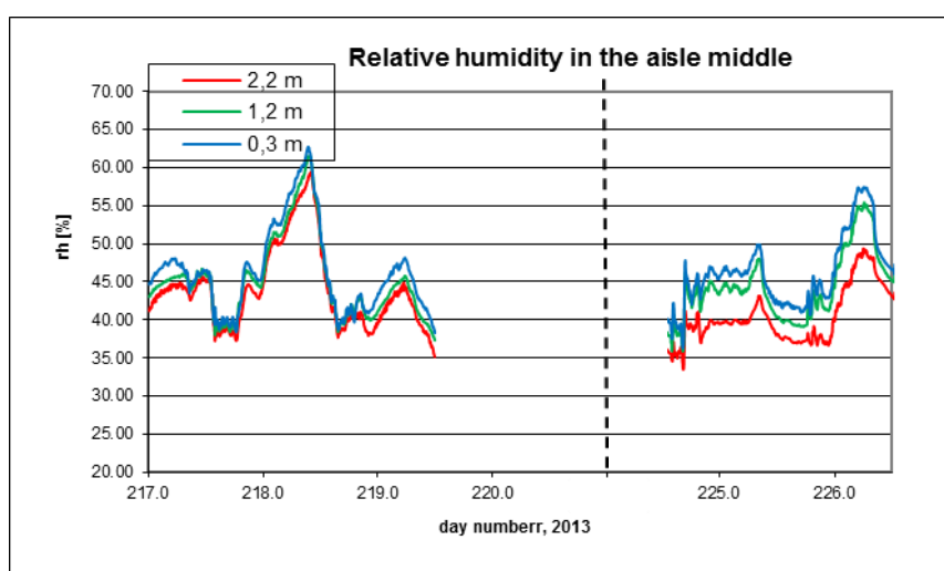
B7.12. Relative humidity in the middle of the aisle.
