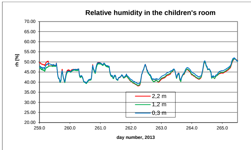
B11.10. Relative humidity in the children's room.
