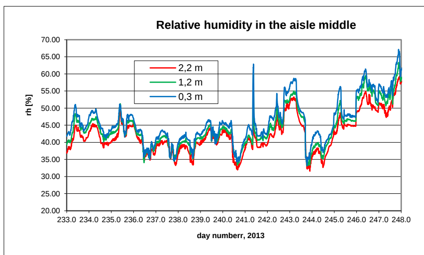
B9.12. Relative humidity in the middle of the aisle.
