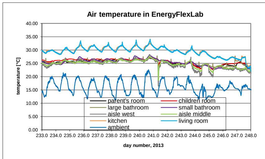
B9.1. Ambient and room temperatures in the house.
