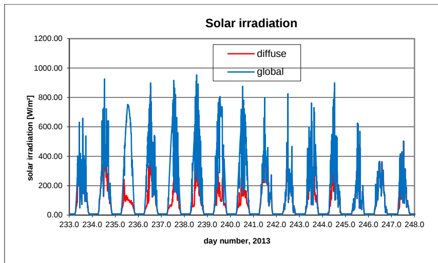
B9.13. Global and diffuse solar radiation.
