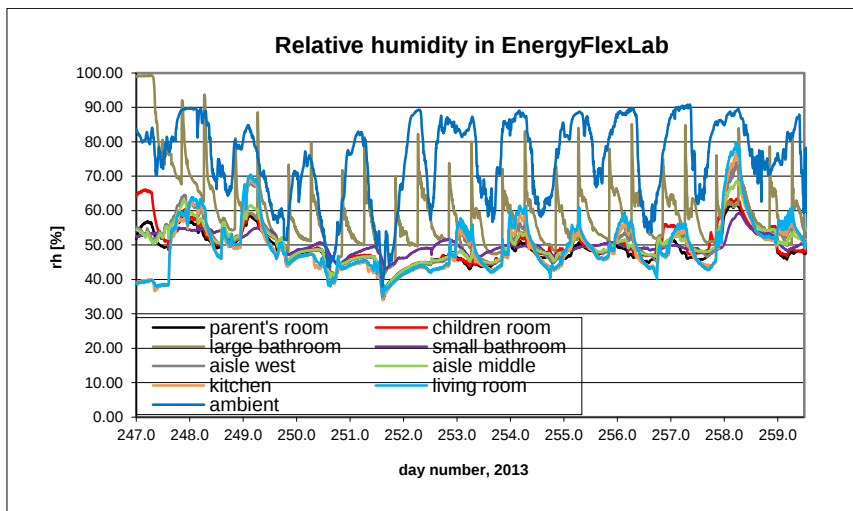
B10.2. Relative humidity in the house and ambient.
