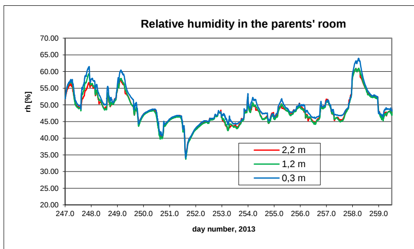
B10.9. Relative humidity in the parents' room.
