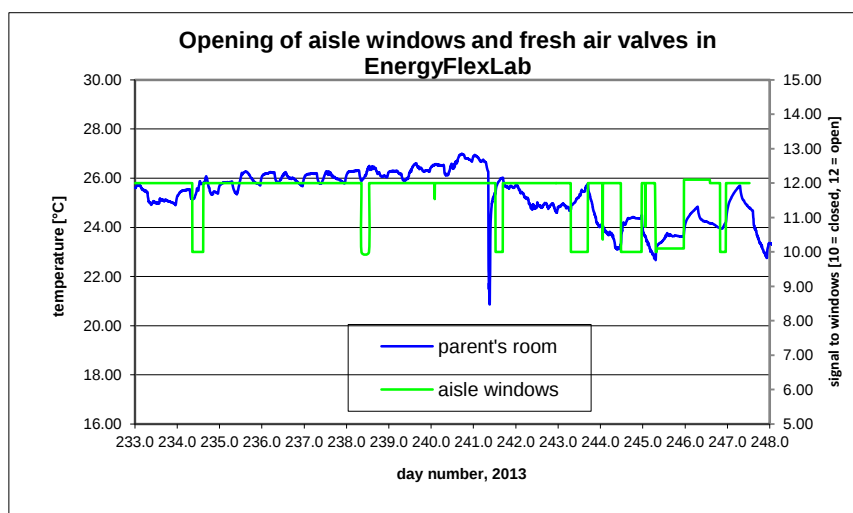
B9.18. Opening of aisle windows and fresh air valves.
