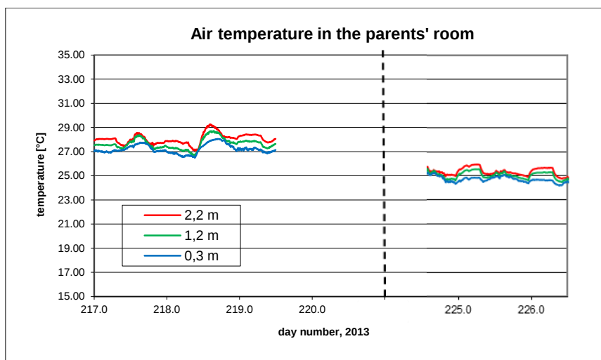
oom temperatures in the parents' room.
