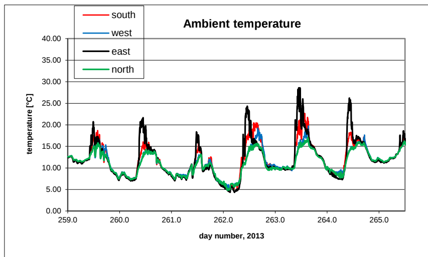
B11.17. Ambient temperature at the facades.
