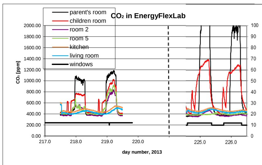
B7.3. CO 2 concentration in the house measured with Vaisala.
