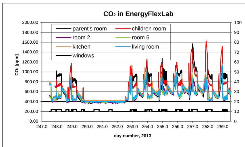
B10.3. CO 2 concentration in the house measured with Vaisala.
