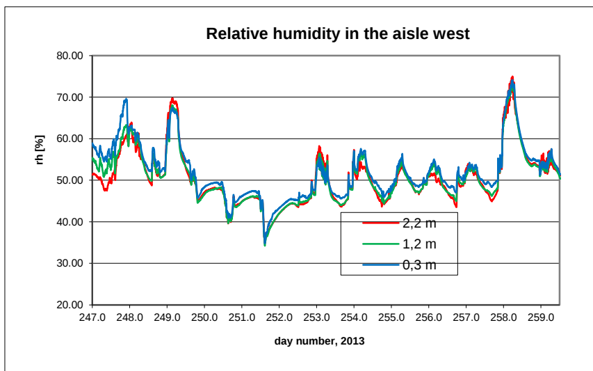
B10.11. Relative humidity in the western part of the aisle.
