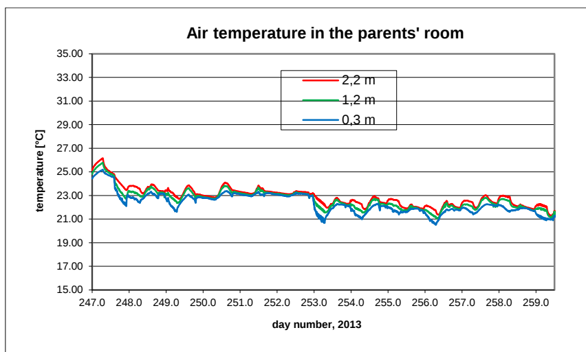
B10.5. Room temperatures in the parents' room.
