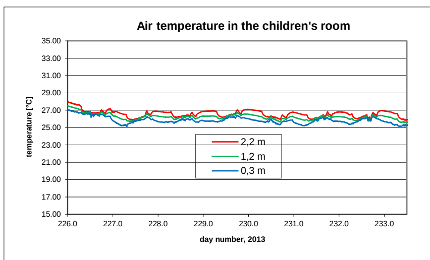
B8.6. Room temperatures in the children's room.
