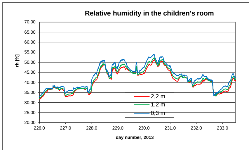
B8.10. Relative humidity in the children's room.
