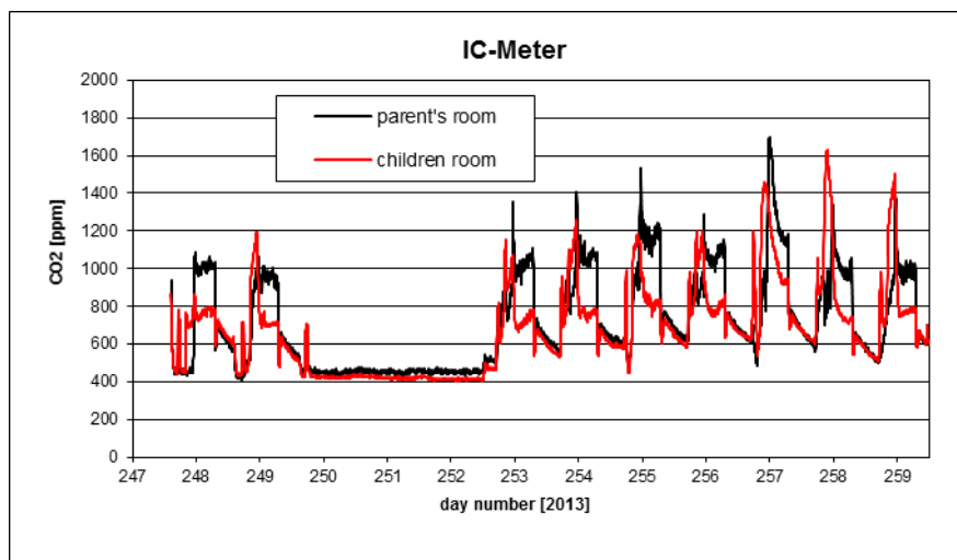
B10.4. CO 2 concentration in the house measured with IC-meters.
