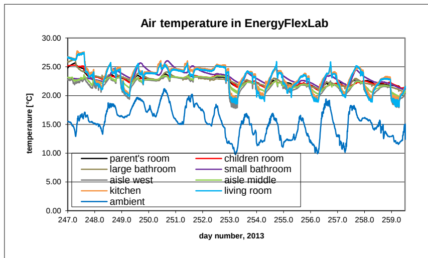
B10.1. Ambient and room temperatures in the house.
