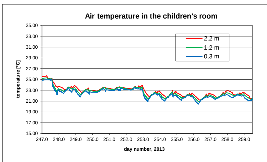
B10.6. Room temperatures in the children's room.
