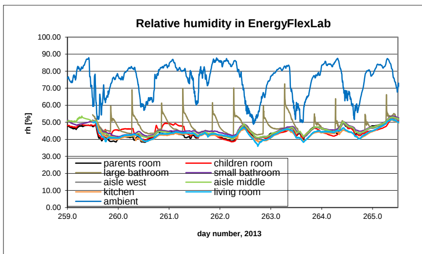
B11.2. Relative humidity in the house and ambient.
