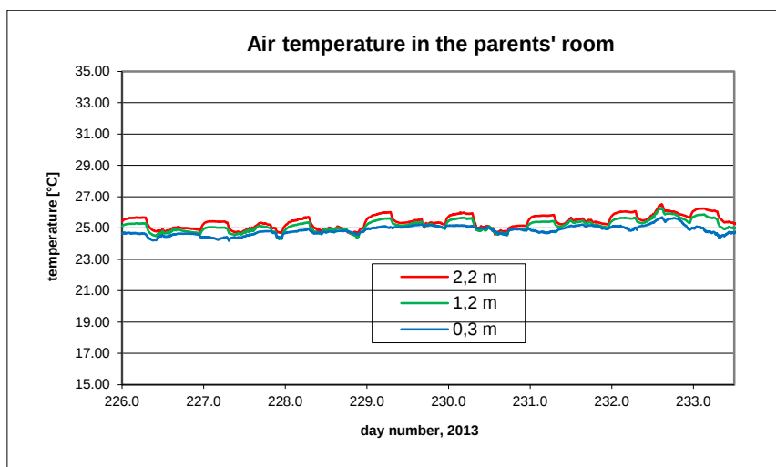
B8.5. Room temperatures in the parents' room.
