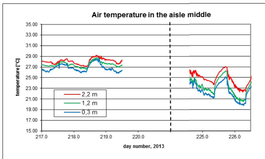
B7.8. Room temperature in the middle of the aisle.
