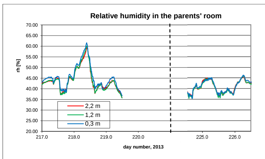
B7.9. Relative humidity in the parents' room.
