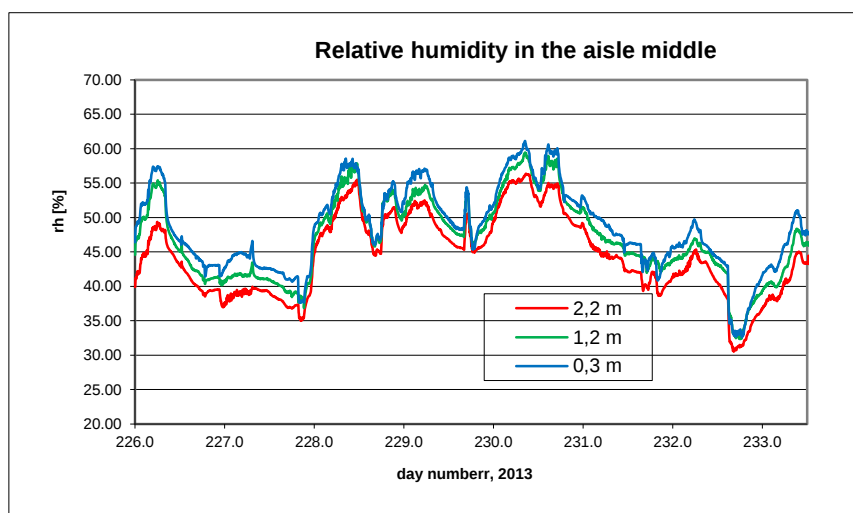
B8.12. Relative humidity in the middle of the aisle.
