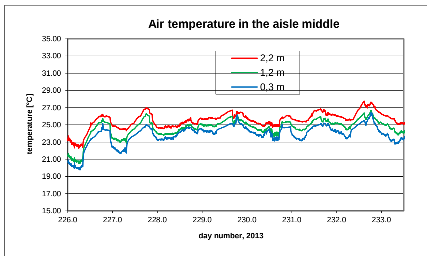
B8.8. Room temperature in the middle of the aisle.
