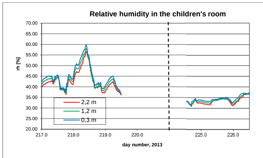
B7.10. Relative humidity in the children's room.
