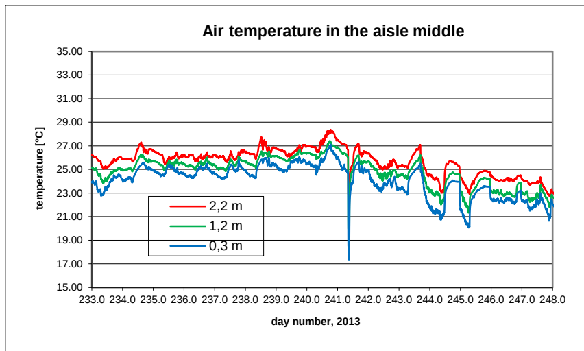
B9.8. Room temperature in the middle of the aisle.
