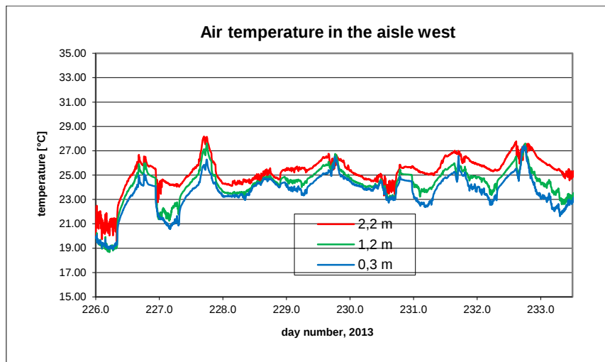
B8.7. Room temperature in the western part of the aisle.
