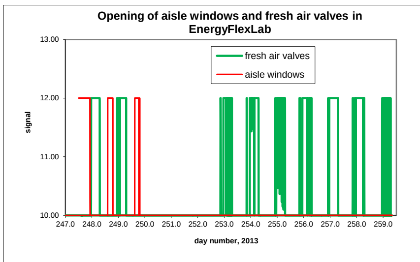
B10.19. Opening of aisle windows and fresh air valves.
