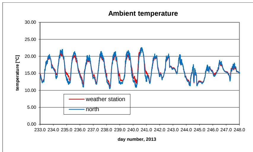
B9.16. Ambient temperature.
