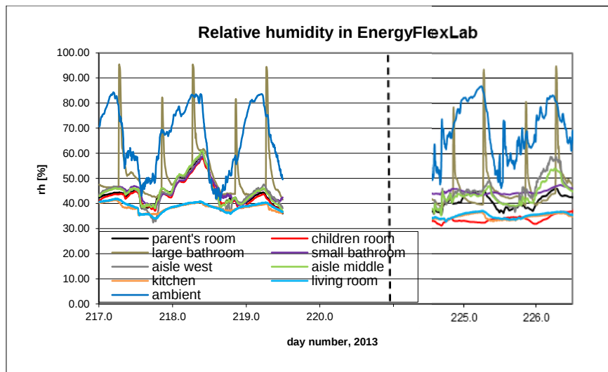
B7.2. Relative humidity in the house and ambient.
