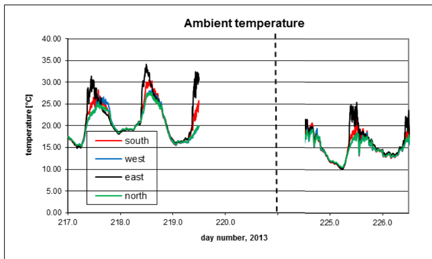
B7.17. Ambient temperature at the facades.
