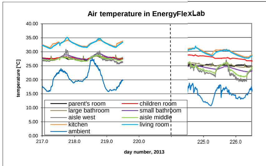
B7.1. Ambient and room temperatures in the house.
