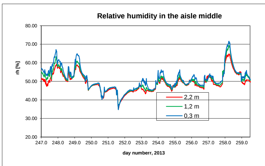
B10.12. Relative humidity in the middle of the aisle.
