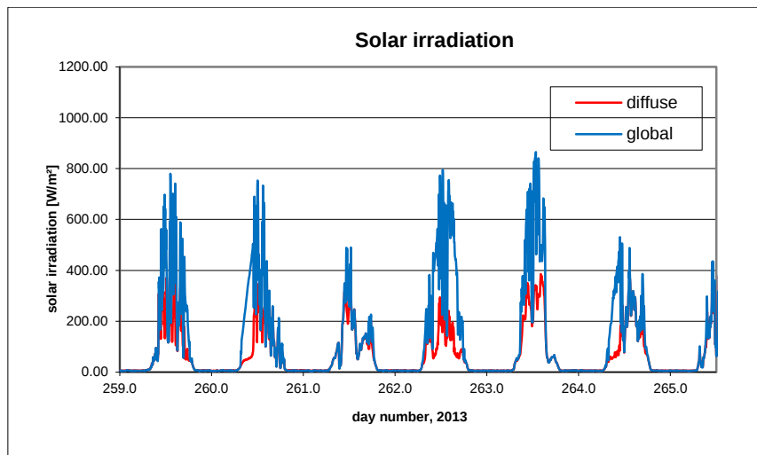
B11.13. Global and diffuse solar radiation.
