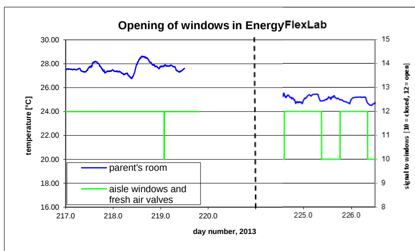
B7.18. Opening of windows.
