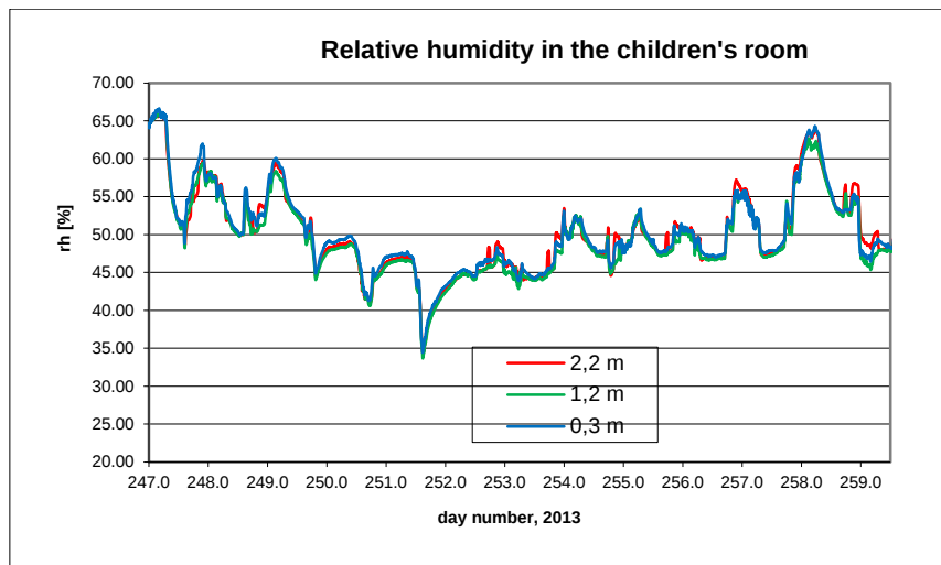
B10.10. Relative humidity in the children's room.
