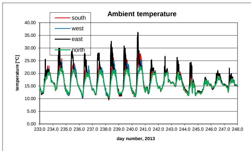
B9.17. Ambient temperature at the facades.
