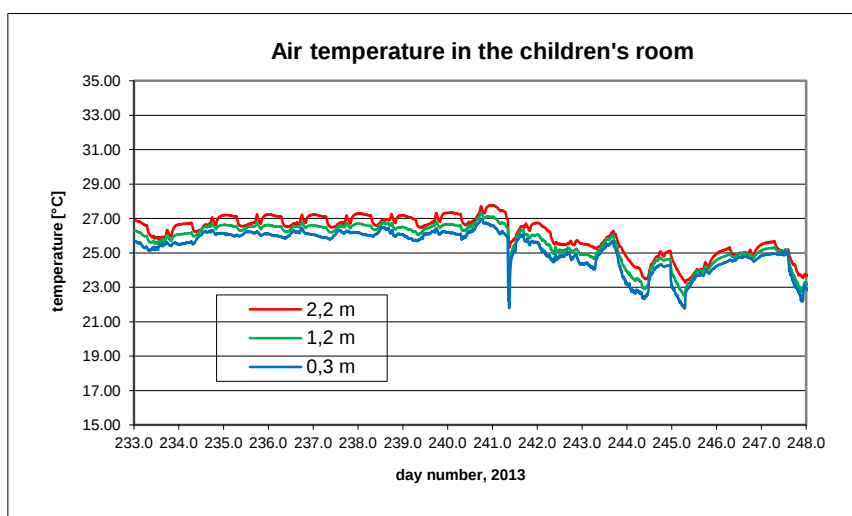
B9.6. Room temperatures in the children's room.
