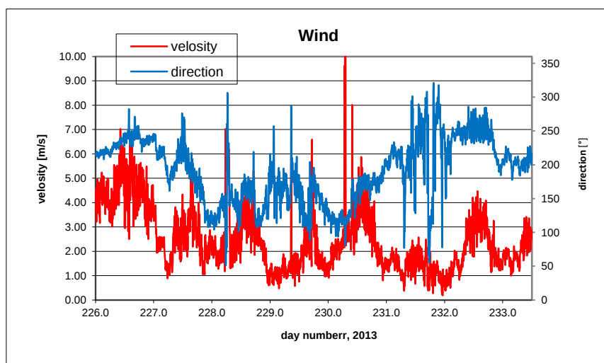
B8.15. Wind direction and wind speed.
