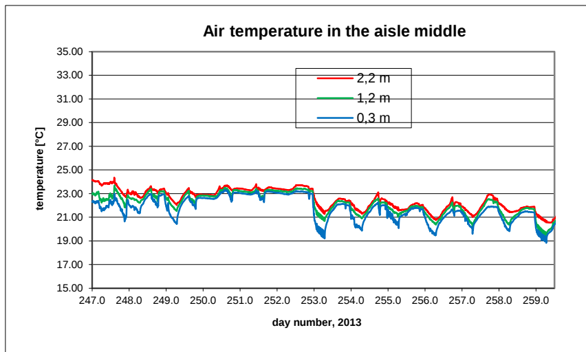
B10.8. Room temperature in the middle of the aisle.
