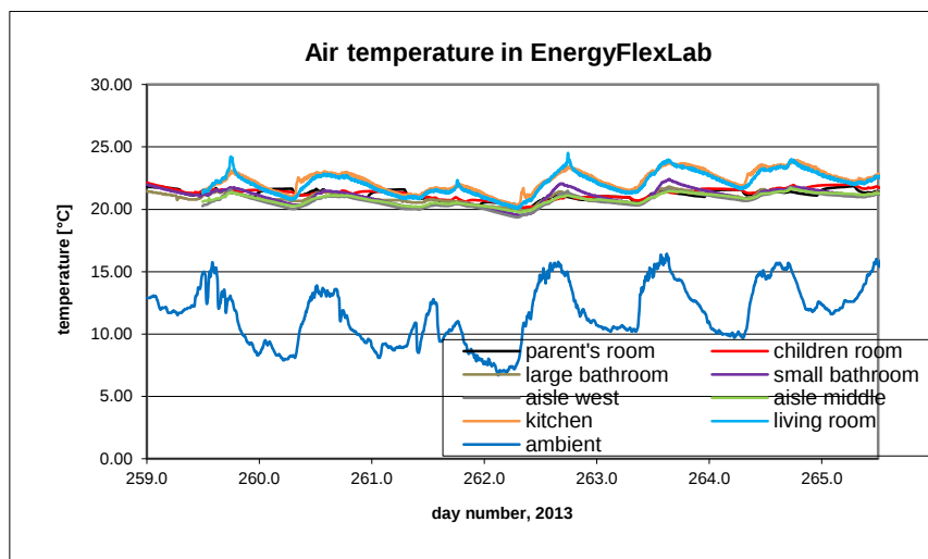
B11.1. Ambient and room temperatures in the house.
