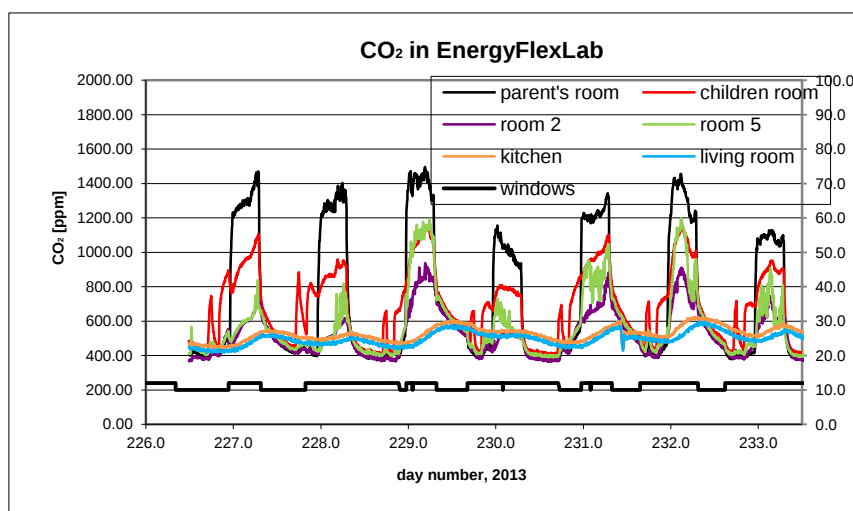
B8.3. CO 2 concentration in the house measured with Vaisala.
