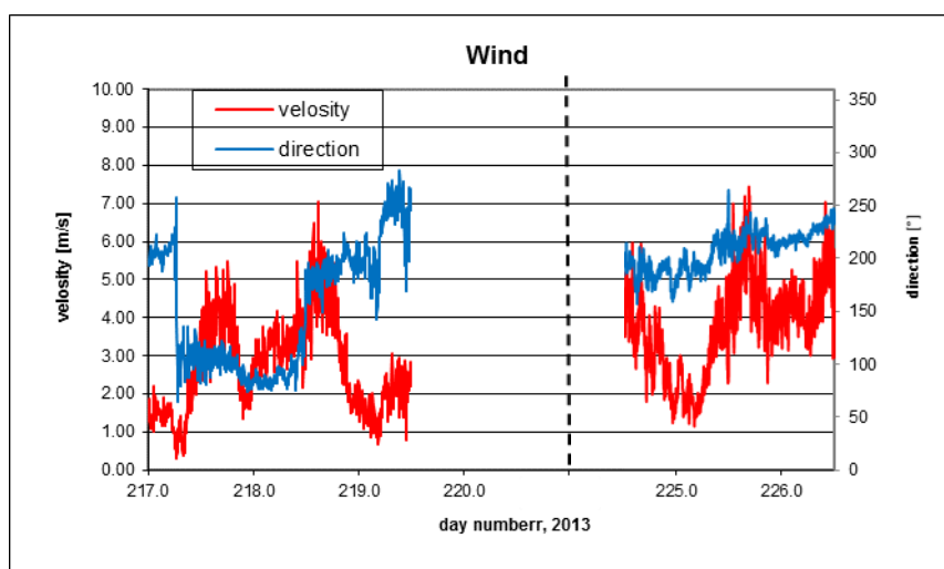
B7.15. Wind direction and wind speed.
