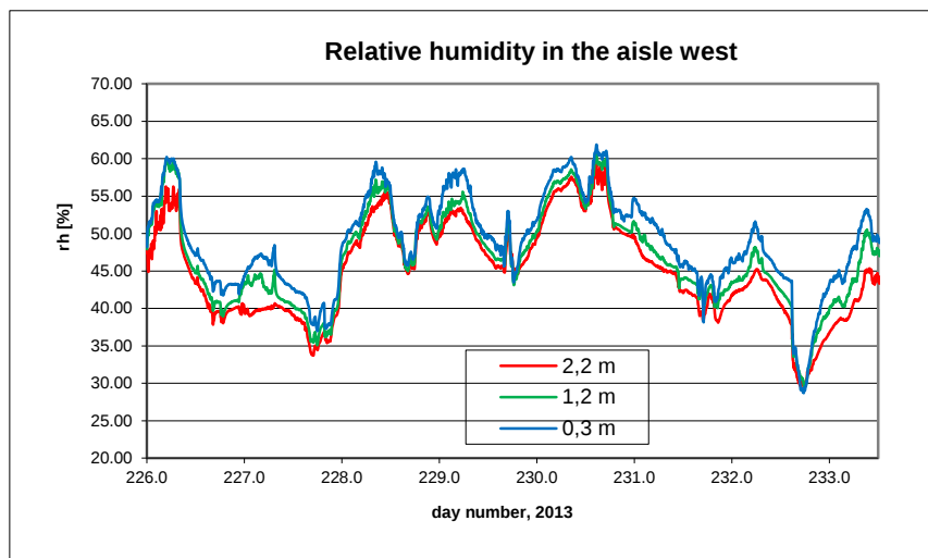
B8.11. Relative humidity in the western part of the aisle.
