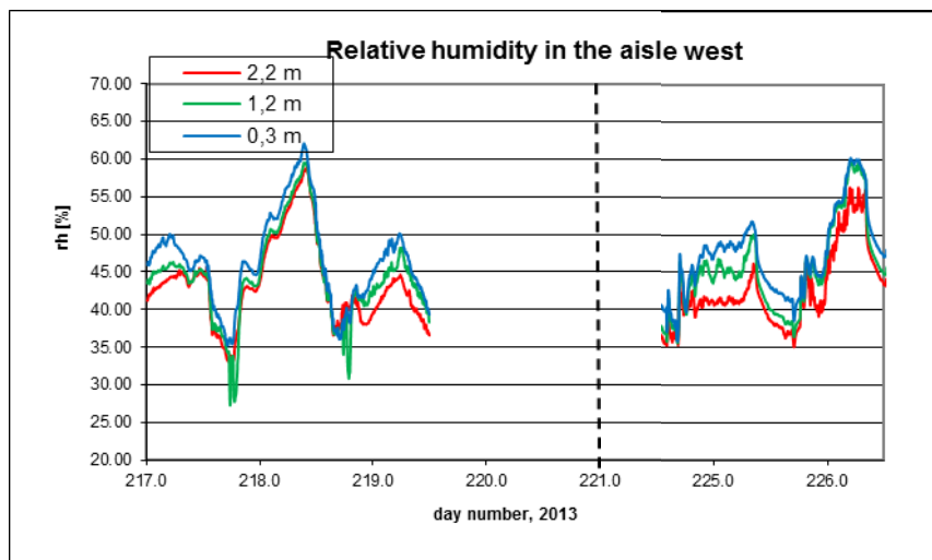
B7.11. Relative humidity in the western part of the aisle.
