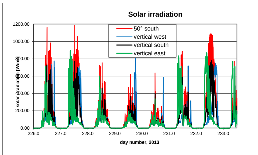
B8.14. Total vertical solar radiations on the facades and on the south facing roof.
