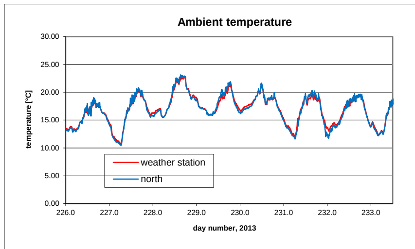
B8.16. Ambient temperature.
