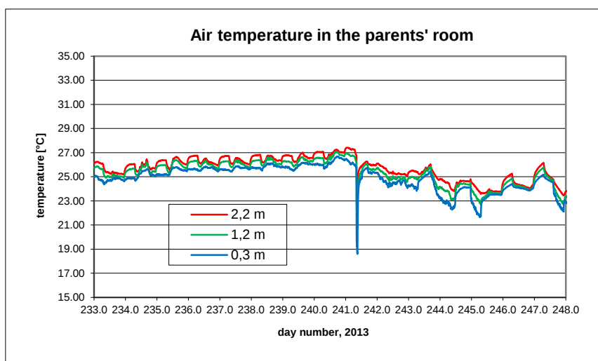
B9.5. Room temperatures in the parents' room.
