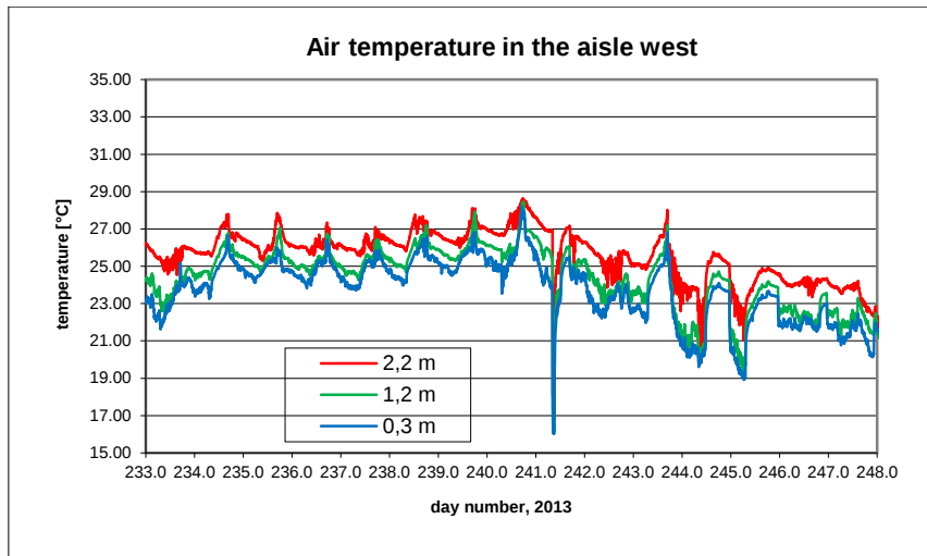
B9.7. Room temperature in the western part of the aisle.
