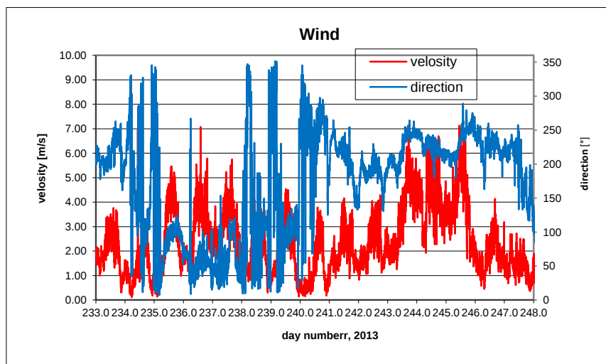
B9.15. Wind direction and wind speed.
