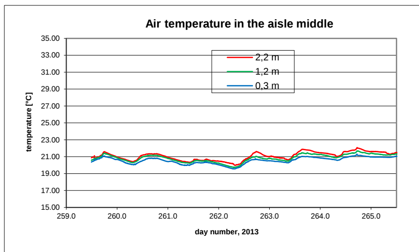
B11.8. Room temperature in the middle of the aisle.
