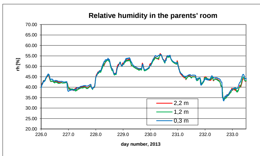
B8.9. Relative humidity in the parents' room.
