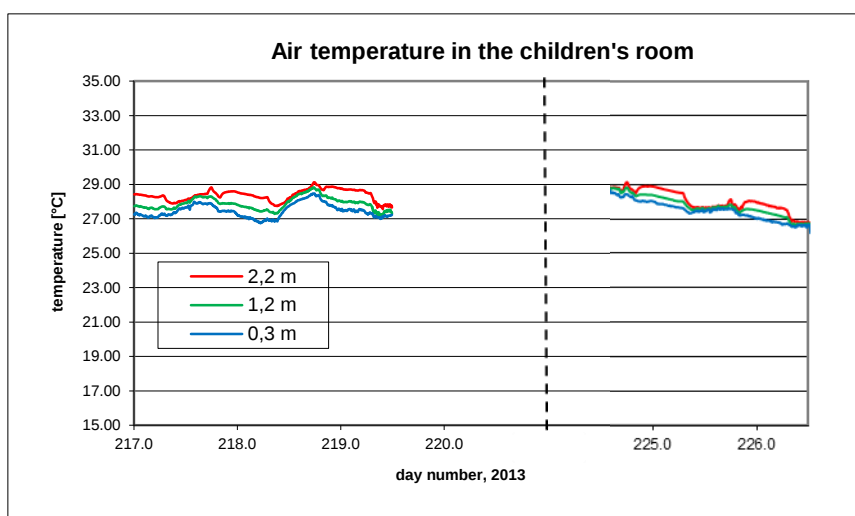
B7.6. Room temperatures in the children's room.
