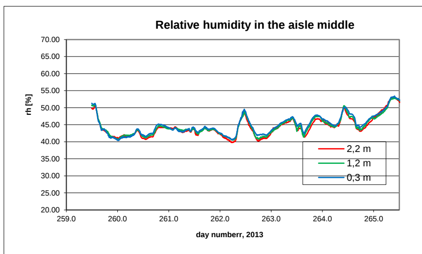
B11.12. Relative humidity in the middle of the aisle.
