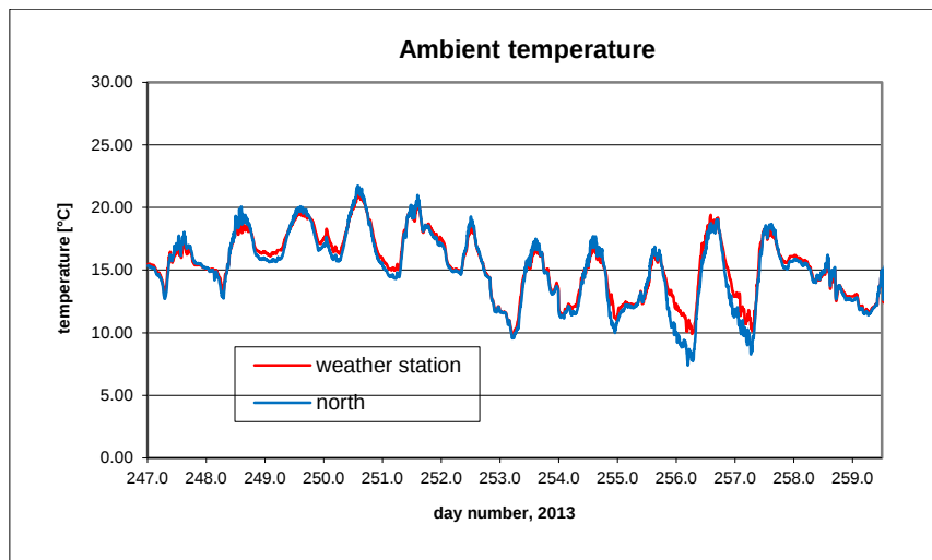
B10.16. Ambient temperature.
