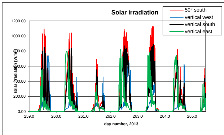
B11.14. Total vertical solar radiations on the facades and on the south facing roof.
