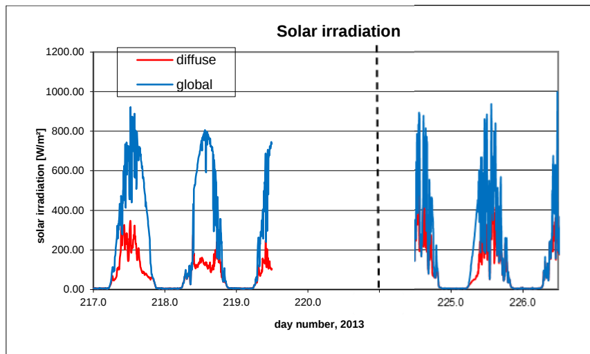
B7.13. Global and diffuse solar radiation.
