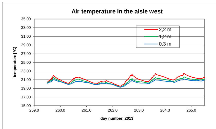
B11.7. Room temperature in the western part of the aisle.
