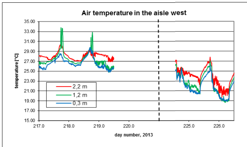
B7.7. Room temperature in the western part of the aisle.
