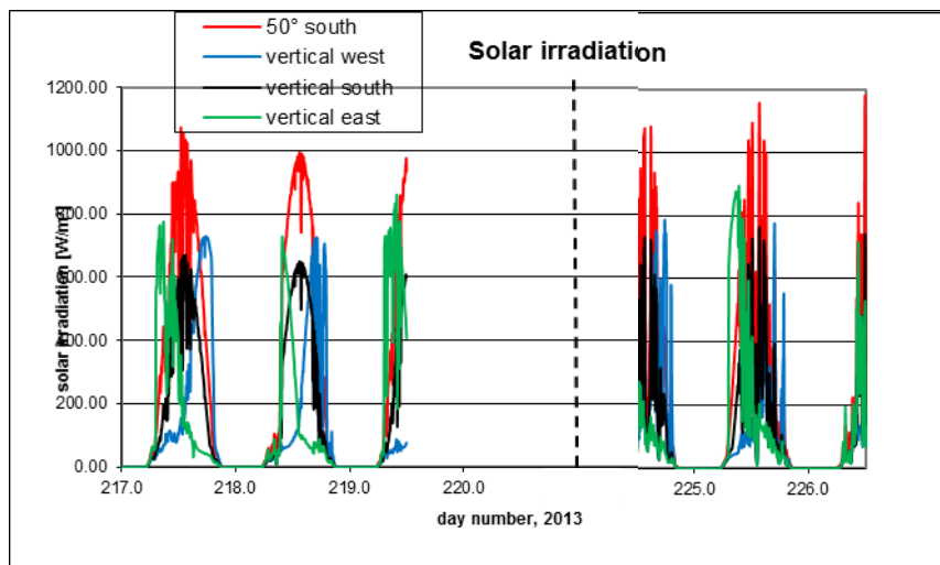
B7.14. Total vertical solar radiations on the facades and on the south facing roof.
