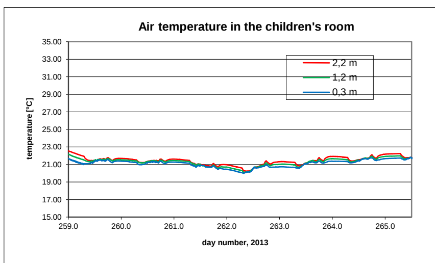
B11.6. Room temperatures in the children's room.
