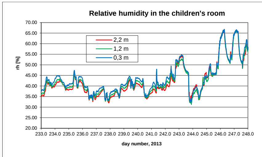
B9.10. Relative humidity in the children's room.
