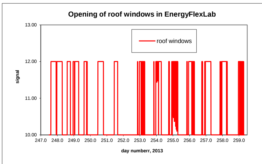
B10.18. Opening of roof windows.
