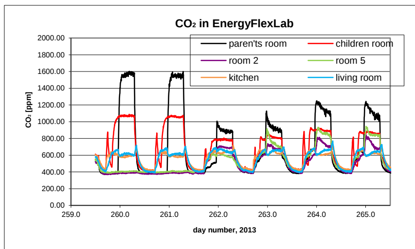
B11.3. CO 2 concentration in the house measured with Vaisala.
