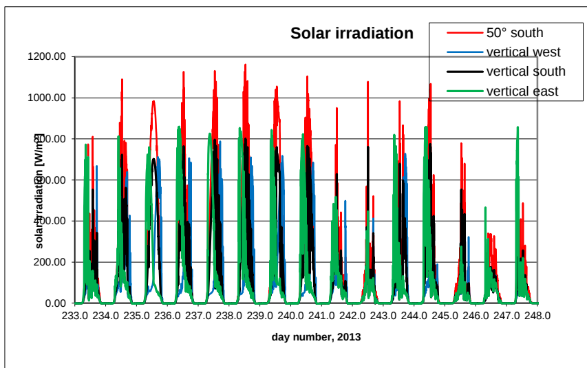
B9.14. Total vertical solar radiations on the facades and on the south facing roof.
