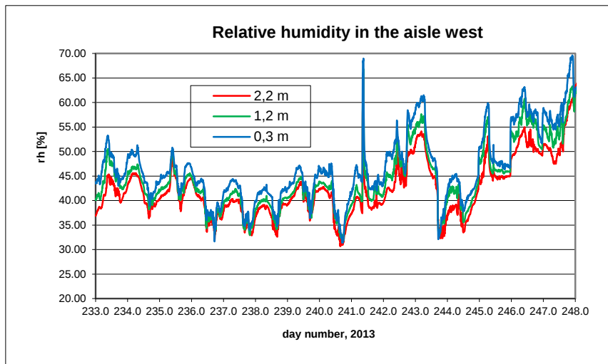
B9.11. Relative humidity in the western part of the aisle.
