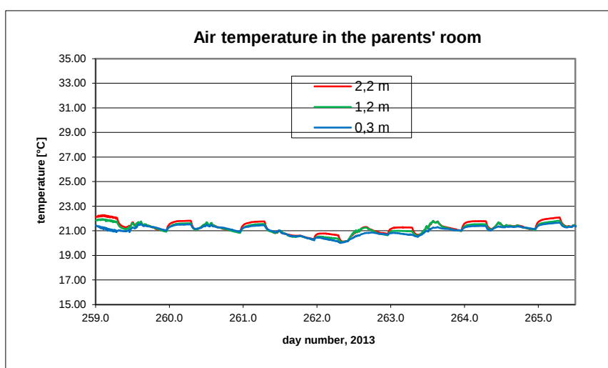
B11.5. Room temperatures in the parents' room.
