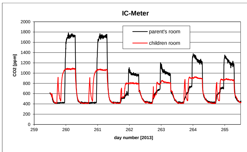
B11.4. CO 2 concentration in the house measured with IC-meters.
