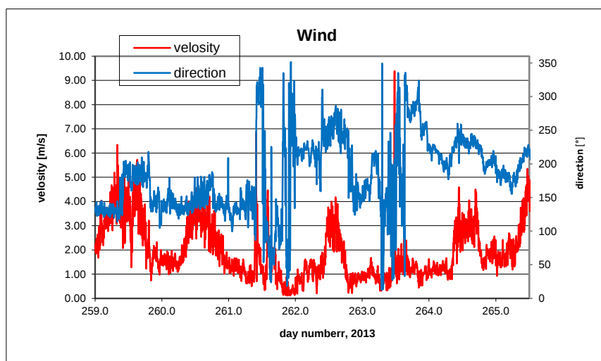
B11.15. Wind direction and wind speed.
