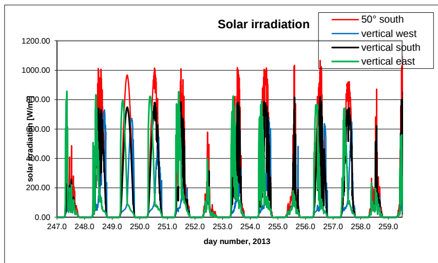
B10.14. Total vertical solar radiations on the facades and on the south facing roof.
