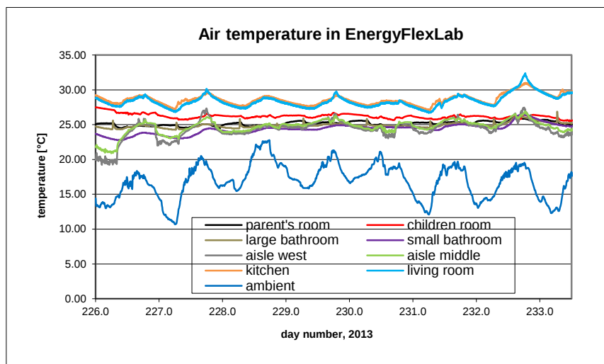
B8.1. Ambient and room temperatures in the house.
