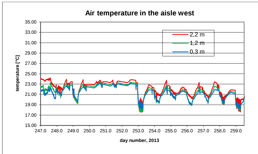
B10.7. Room temperature in the western part of the aisle.
