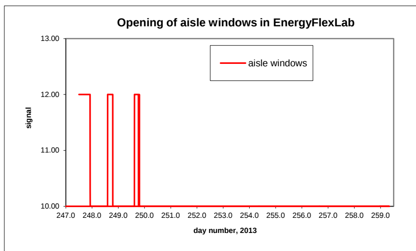
B10.20. Opening of aisle windows.
