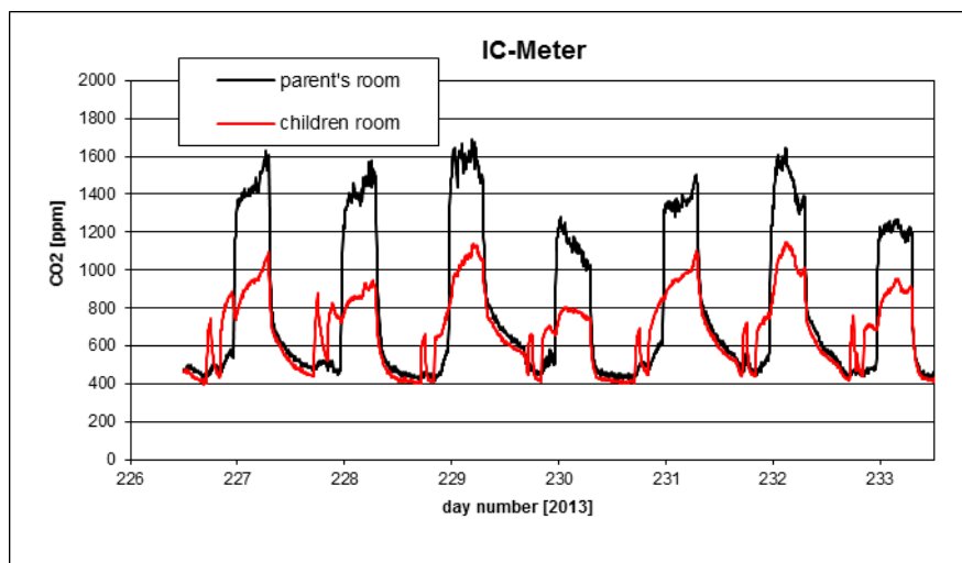
B8.4. CO 2 concentration in the house measured with IC-meters.
