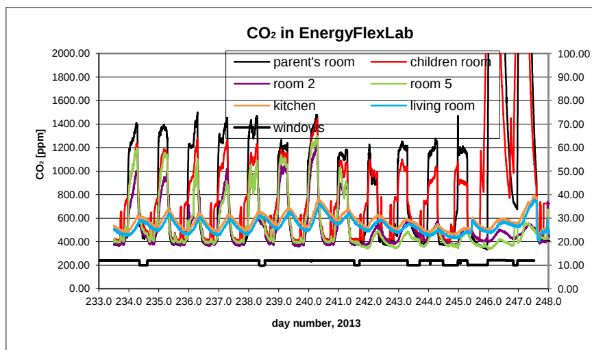
B9.3. CO 2 concentration in the house measured with Vaisala.
