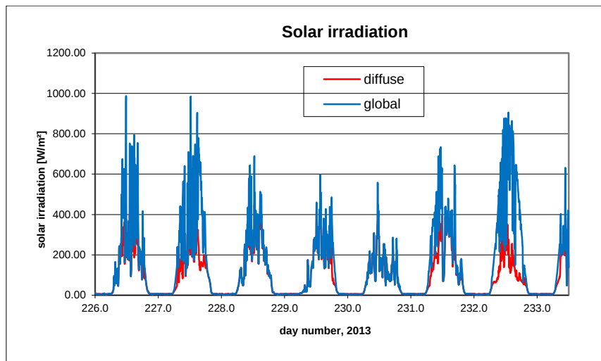
B8.13. Global and diffuse solar radiation.
