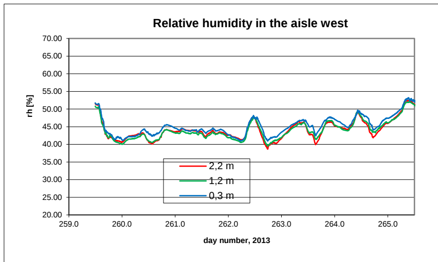
B11.11. Relative humidity in the western part of the aisle.
