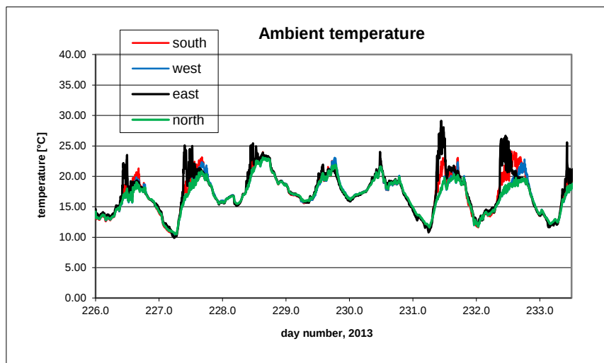
B8.17. Ambient temperature at the facades.
