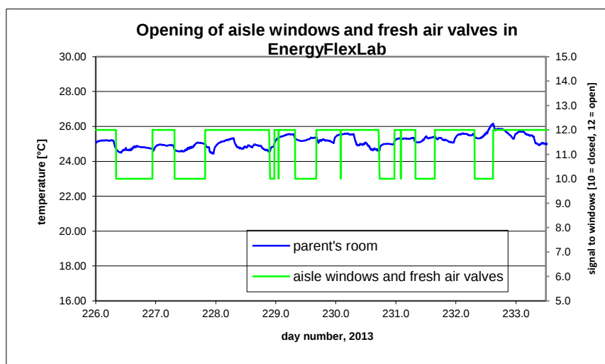
B8.18. Opening of aisle windows and fresh air valves.
