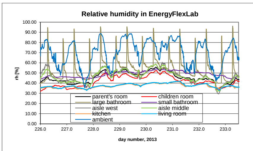
B8.2. Relative humidity in the house and ambient.
