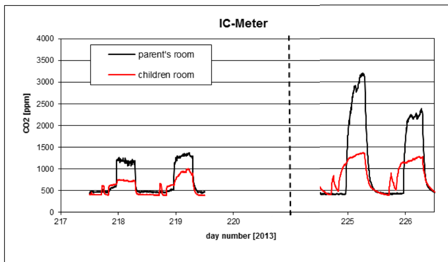
B7.4. CO 2 concentration in the house measured with IC-meters.
