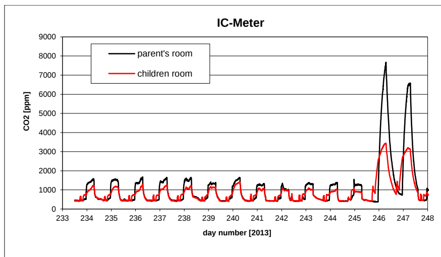
B9.4. CO 2 concentration in the house measured with IC-meters.
