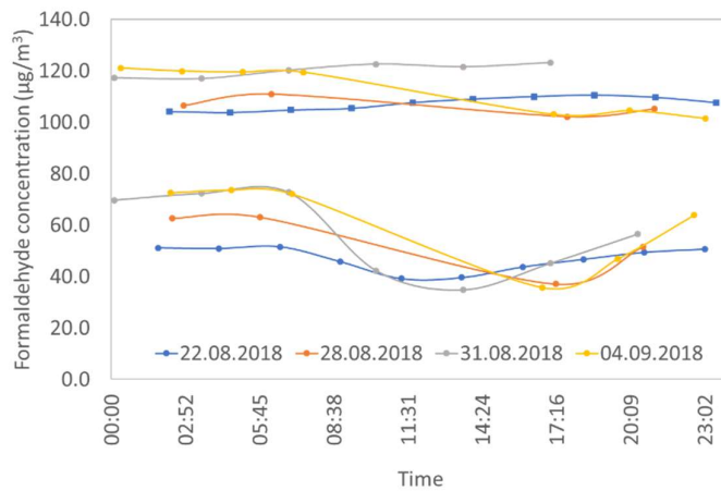
Figur 1. The plot below merely illustrates the semi-quantitative trend of formaldehyde emission during the four measuring days in the test period in the reference chamber (squares) and in the plant chamber (circles). Symbols indicate measuring time points.
