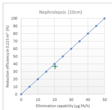
Figure 2: The trendline represent all plants tested. Green circle represents mean and standard error for three replicates of Nephrolepis exaltata . EC is the capacity at ~ 100 \mu\text{g FA}/\text{m}^3 . RE is the effect in the measuring conditions.
