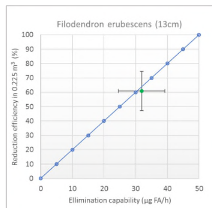
Figure 2: The trendline represent all plants tested. Green circle represents mean and standard error for three replicates of Filodendron erubescens . EC is the capacity at ~ 100 \mu\text{g FA}/\text{m}^3 . RE is the effect in the measuring conditions.
